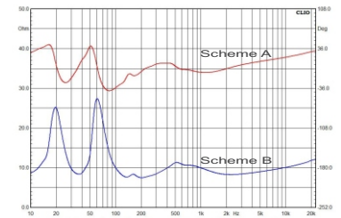
Crossover scheme A - with capacitor Crossover scheme B - without capacitor
